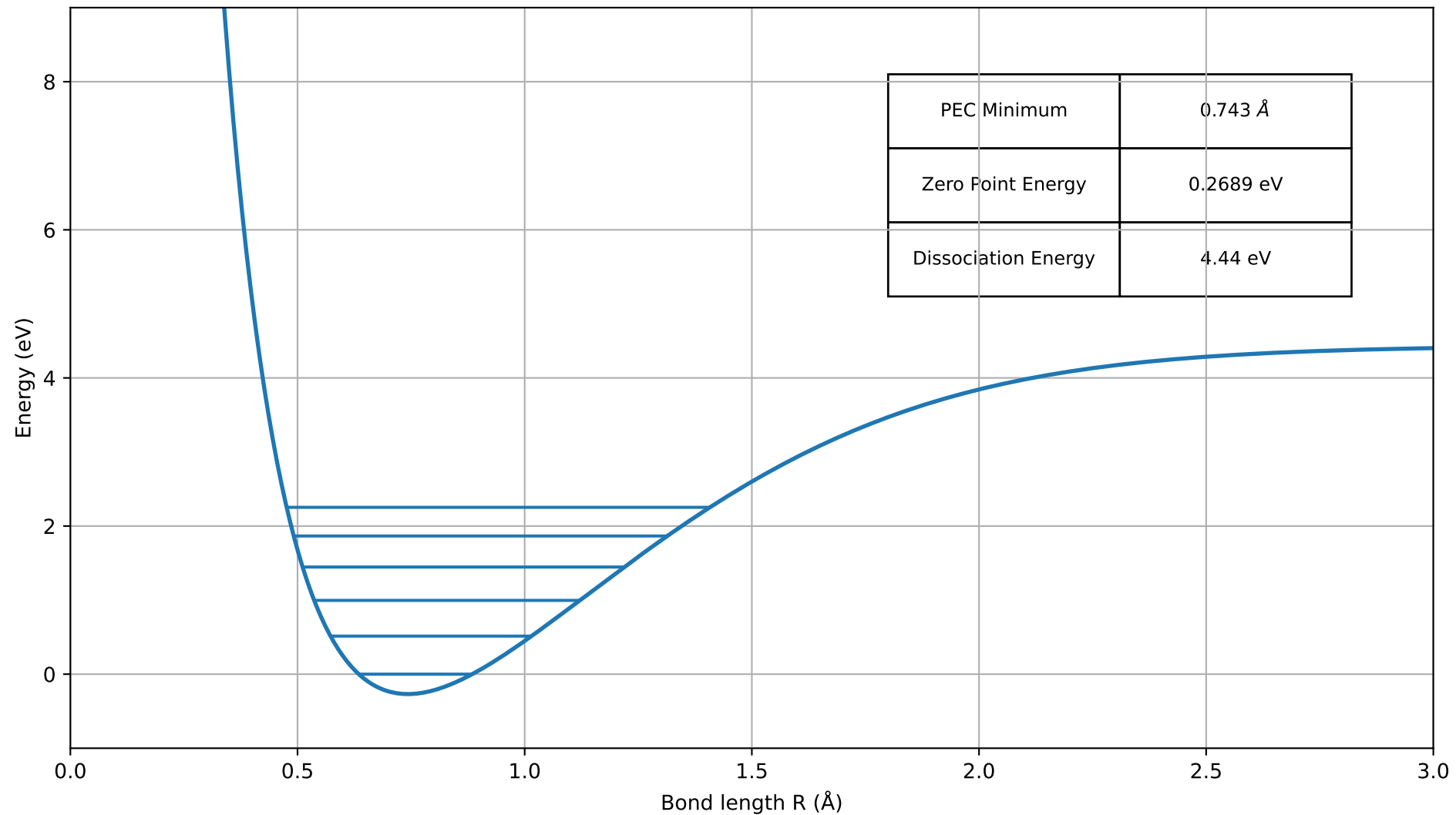
H 2 Ground State PEC and Vibrational Energies
